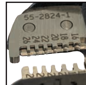
High precision counter-bored razor type blades gauge 16-26AWG
